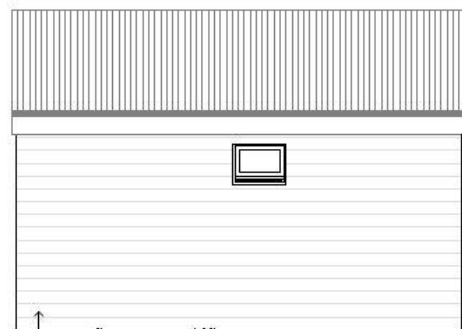
16 Back Elevation 1:100
