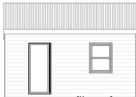
14 Front Elevation 1:100
